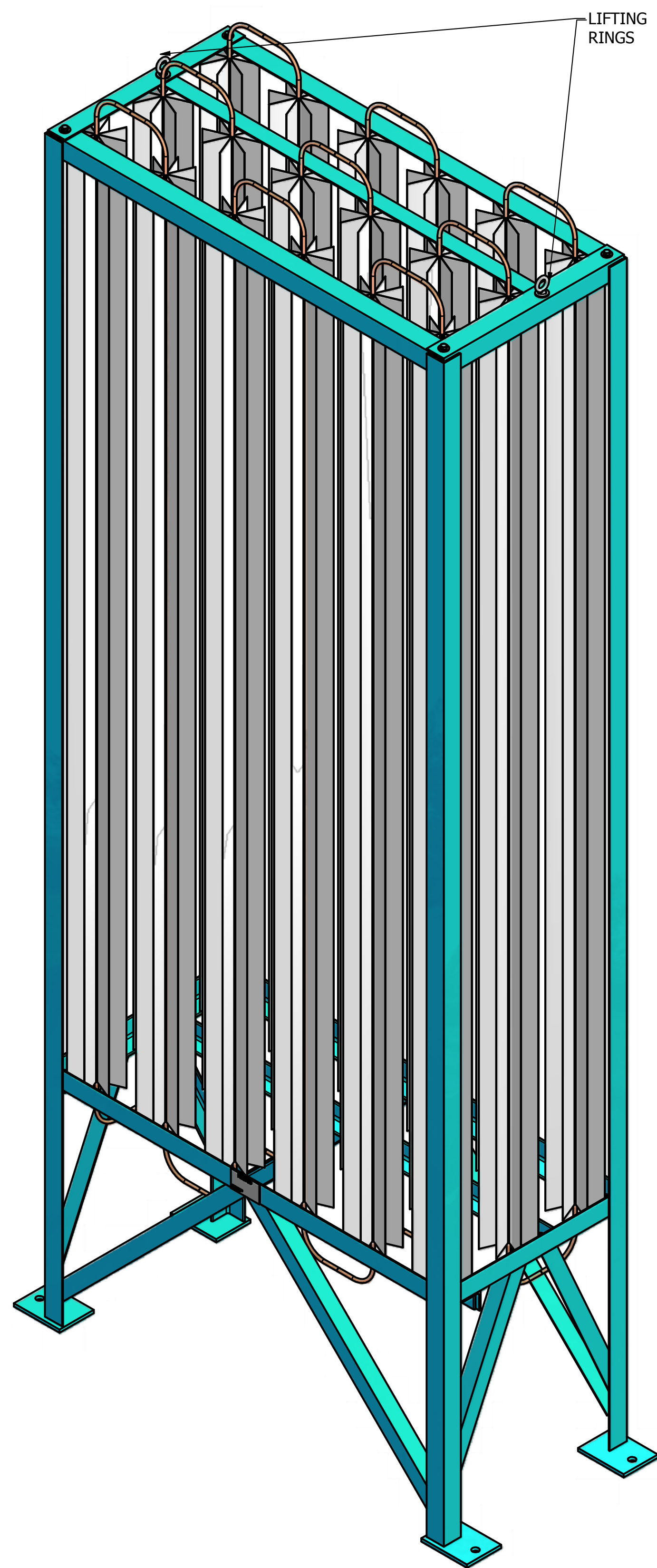
ISOMETRIC VIEW
