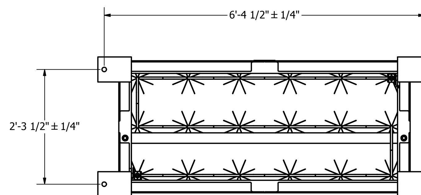
FOUNDATION BOLT PATTERN
