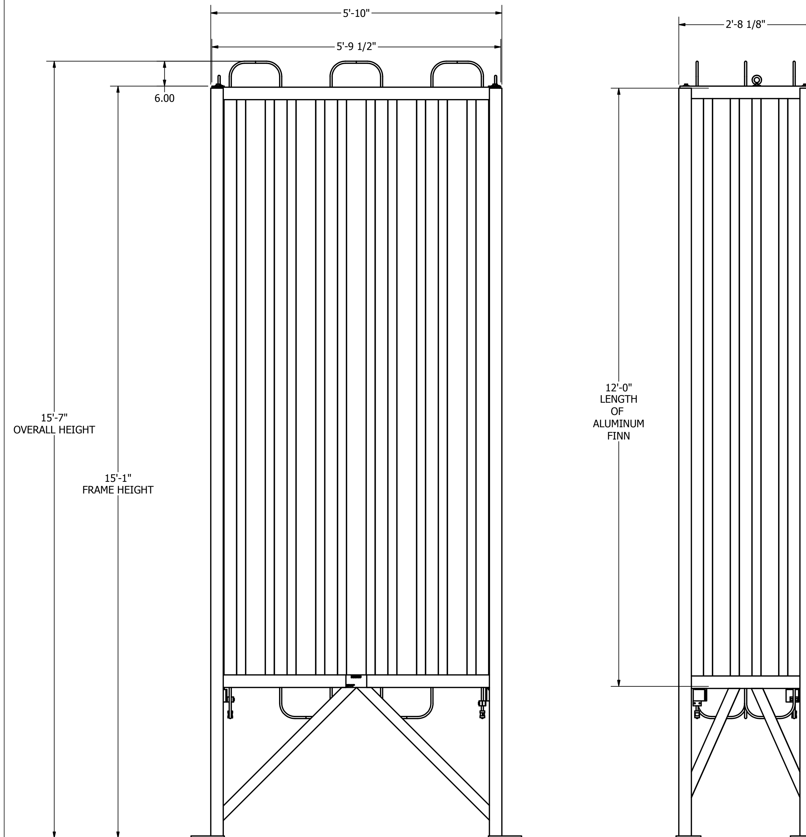
FRONT VIEW
